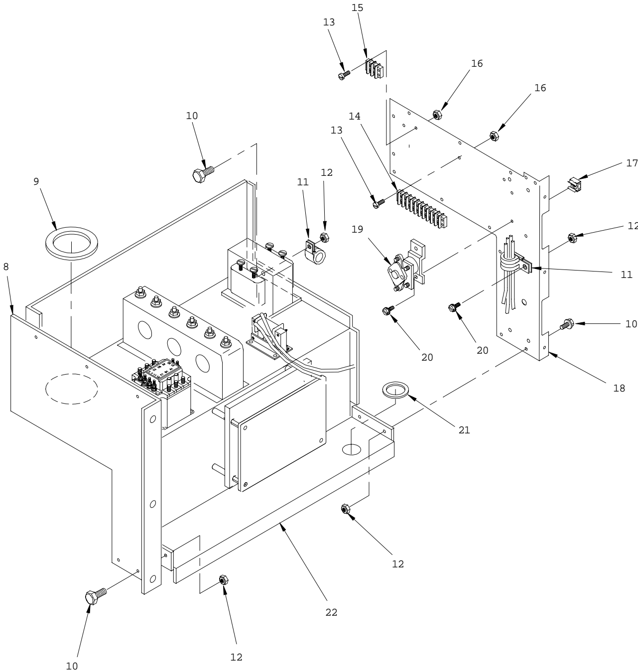
Figure 14. Output Box Assembly (Sheet 2 of 3)
