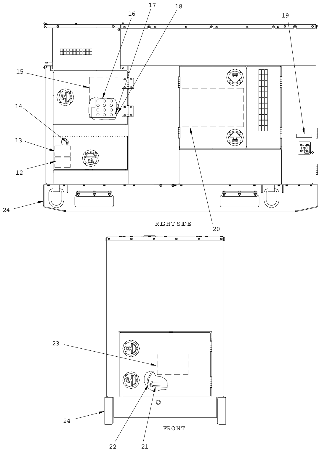
Figure 1. Generator Set, 30 KW (Sheet 2 of 2)
