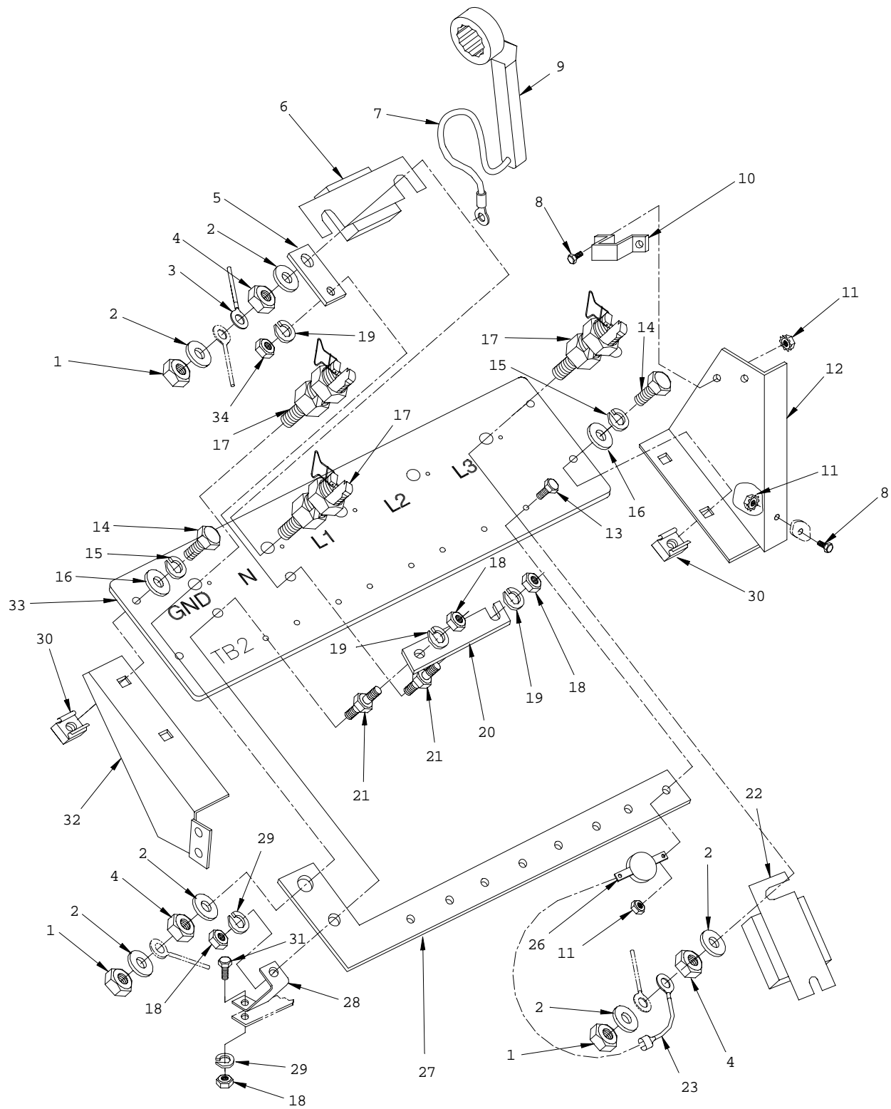
Figure 17. Load Output Terminal Board Assembly
