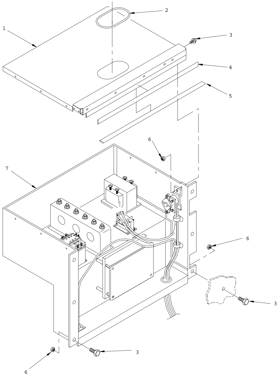
Figure 14. Output Box Assembly (Sheet 1 of 3)
