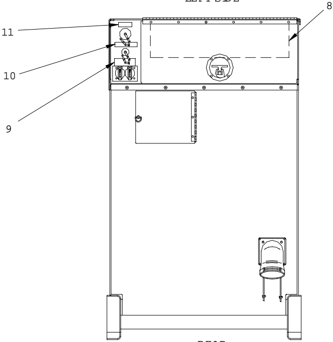
Figure 1. Generator Set, 30 KW (Sheet 1 of 2)
