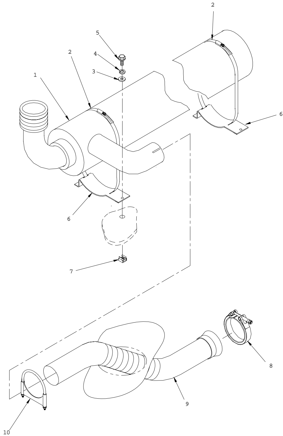
Figure 7. Air Intake and Exhaust System (Sheet 1 of 3)
