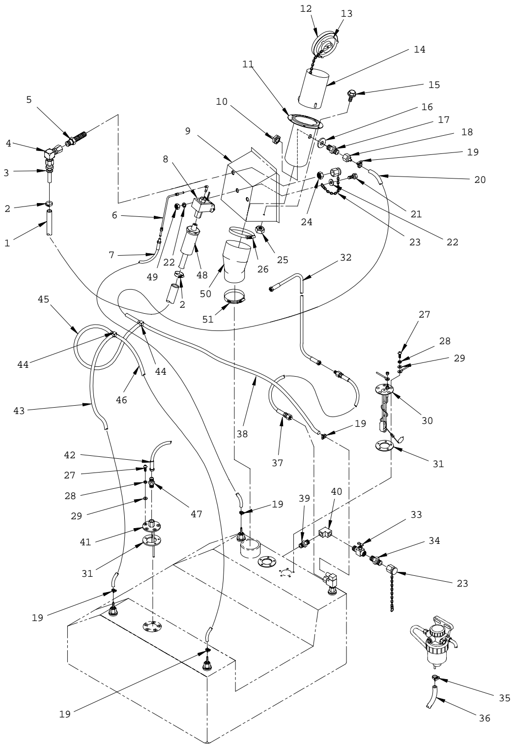
Figure 11. Fuel System (Sheet 1 of 3)
