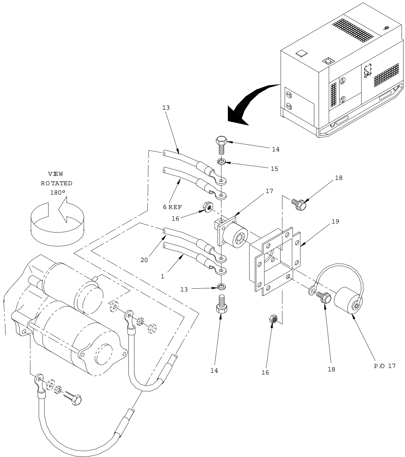
Figure 2. DC Electrical System (Sheet 2 of 2)
