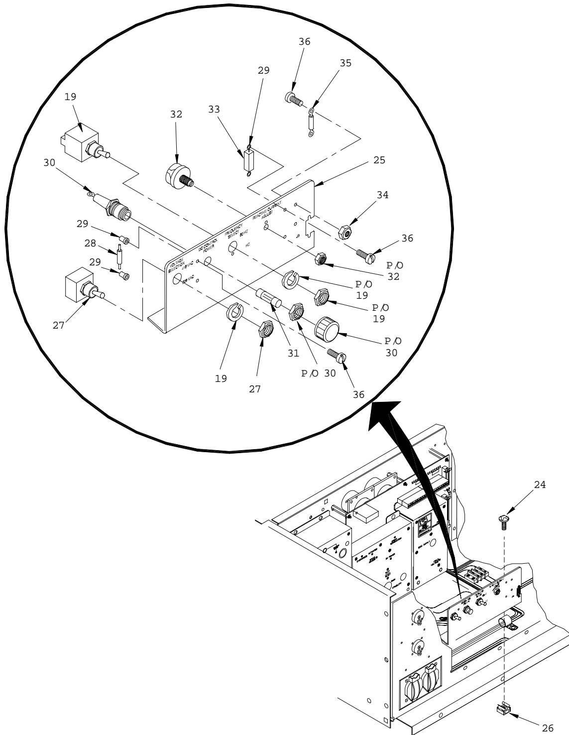
Figure 5. DCS Control Box Assembly (Sheet 5 of 11)
