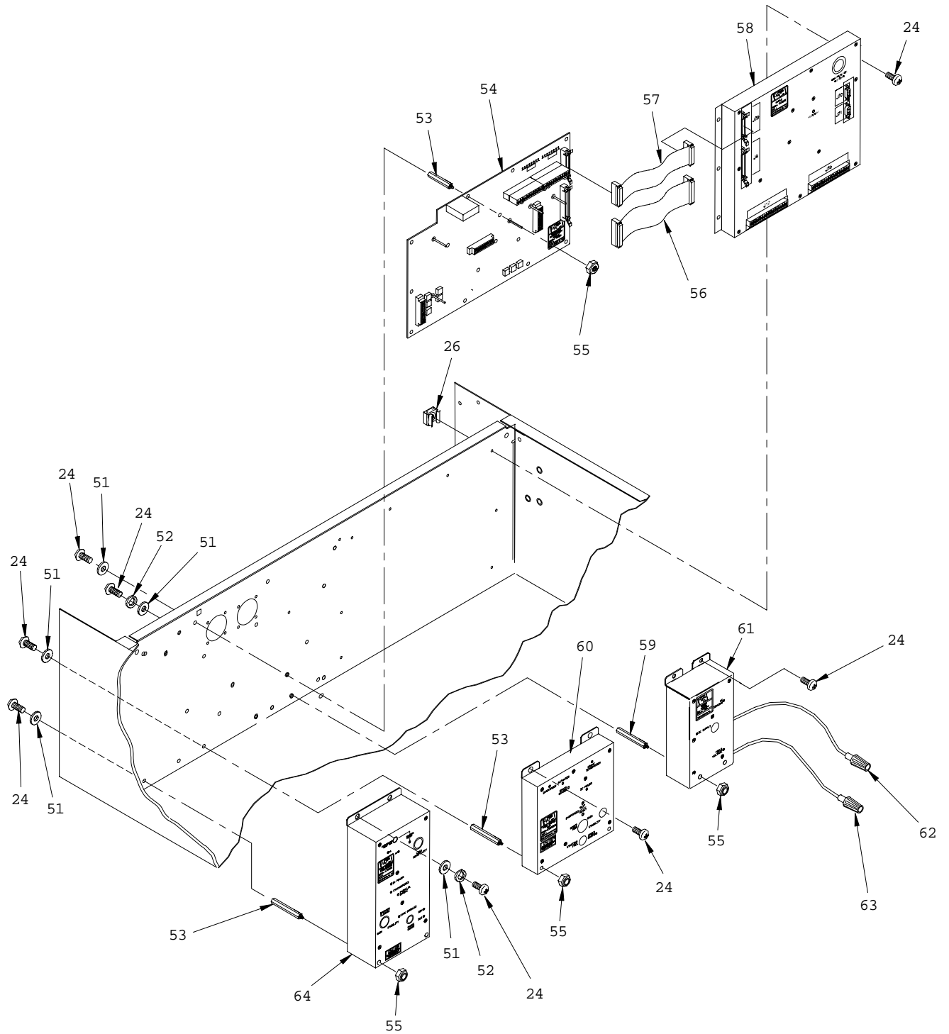
Figure 5. DCS Control Box Assembly (Sheet 7 of 11)
