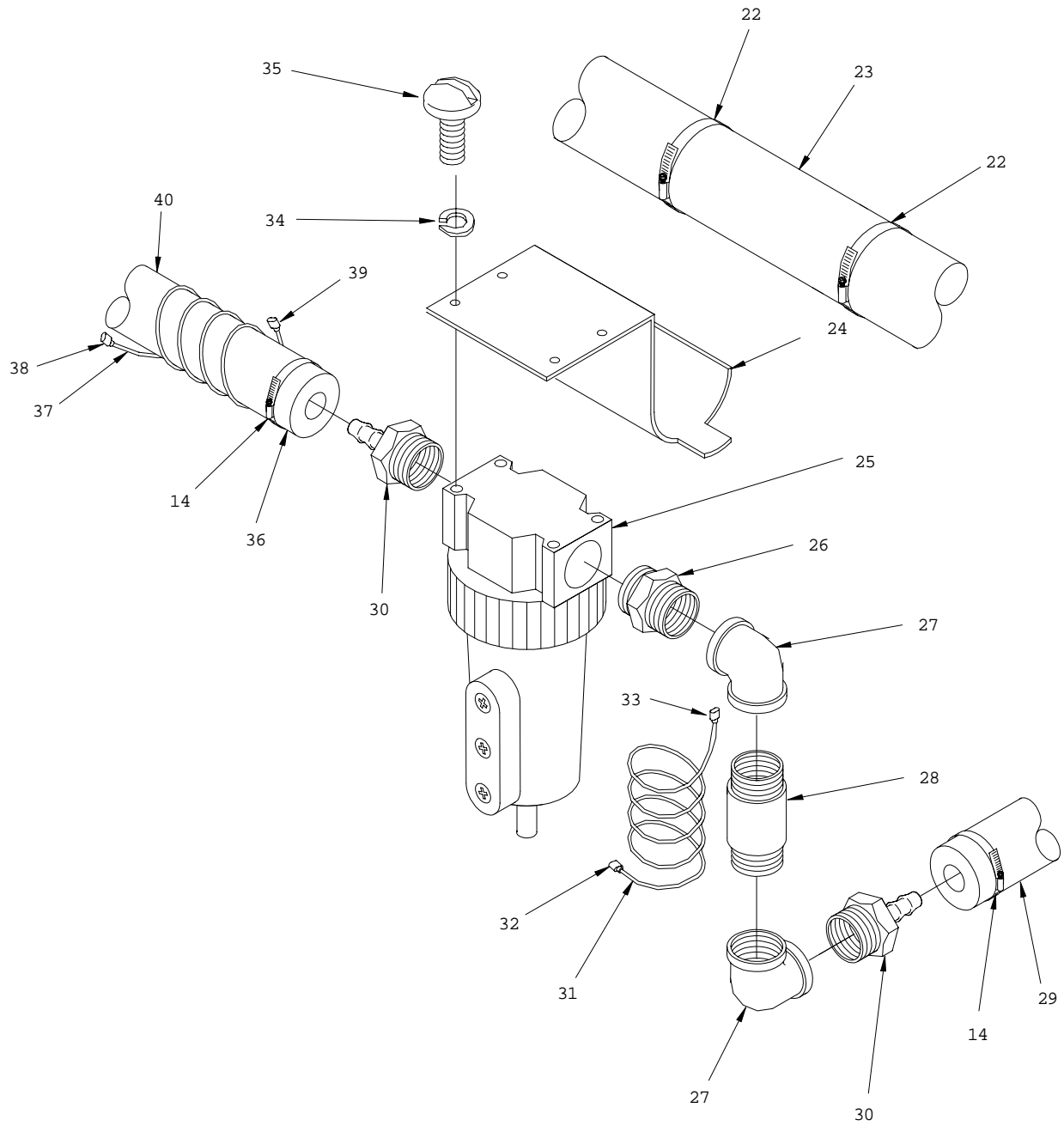
Figure 7. Air Intake and Exhaust System (Sheet 3 of 3)
