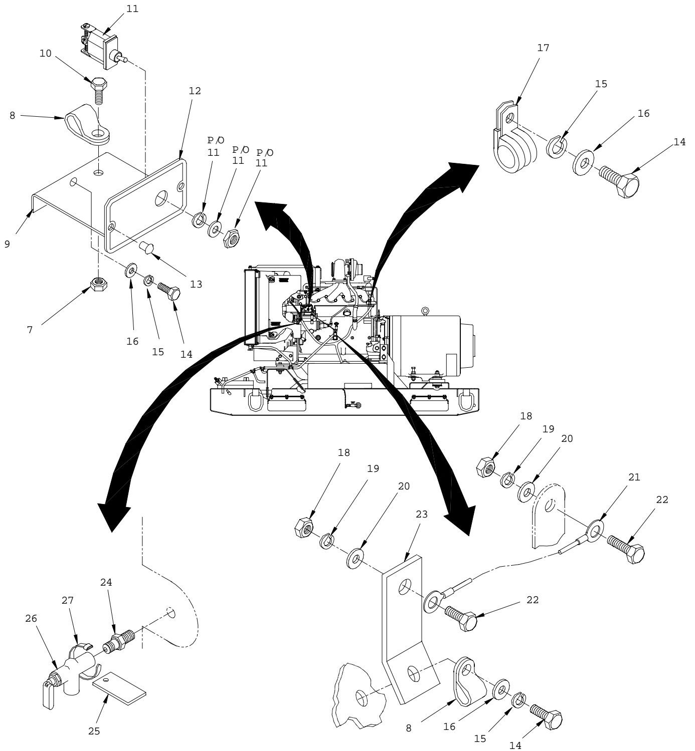
Figure 19. Engine Accessories (Sheet 2 of 4)
