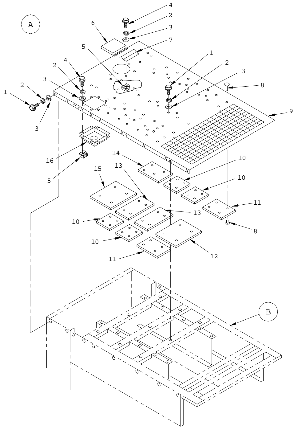
Figure 4. Housing (Sheet 2 of 10)
