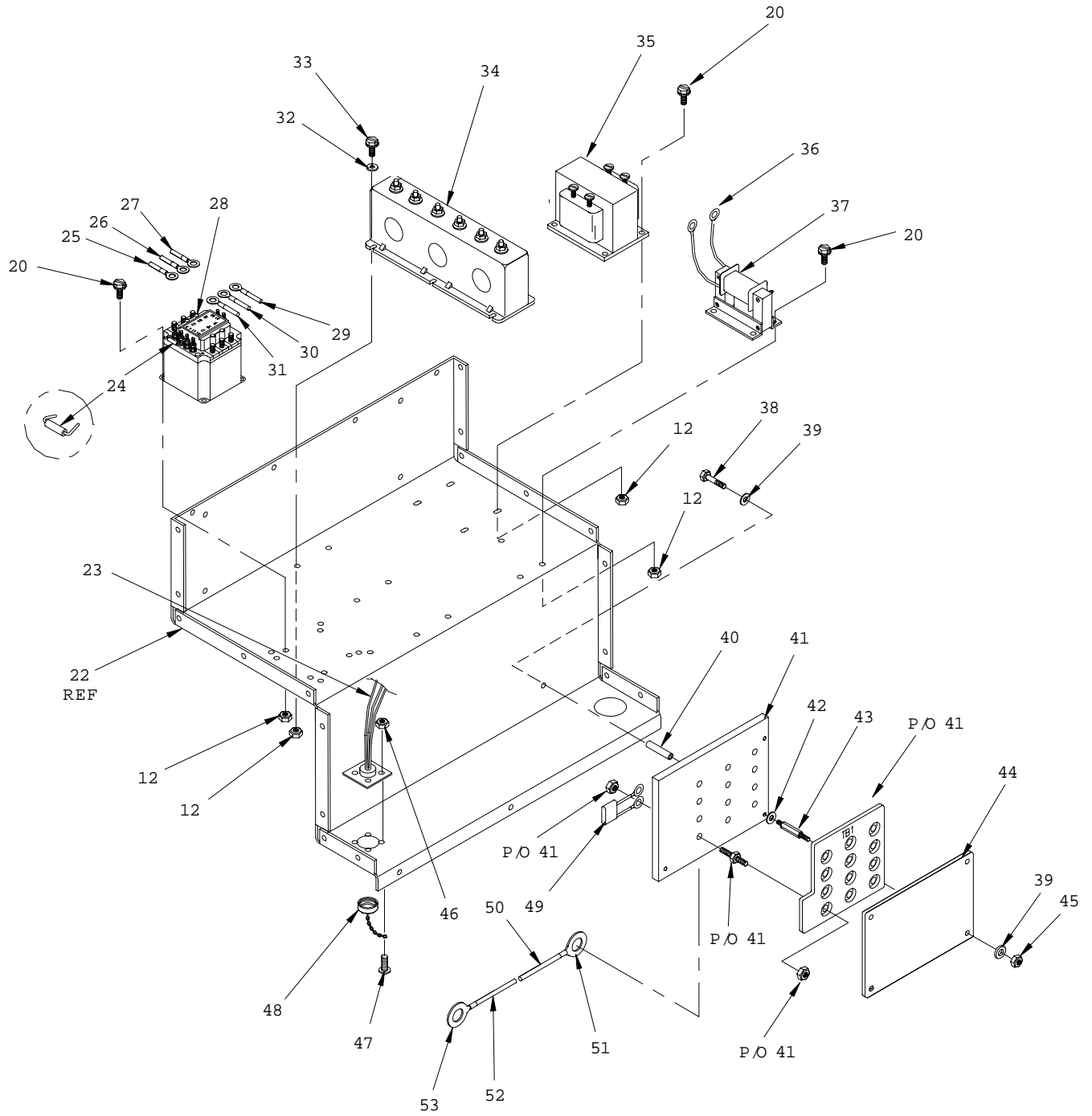
Figure 14. Output Box Assembly (Sheet 3 of 3)
