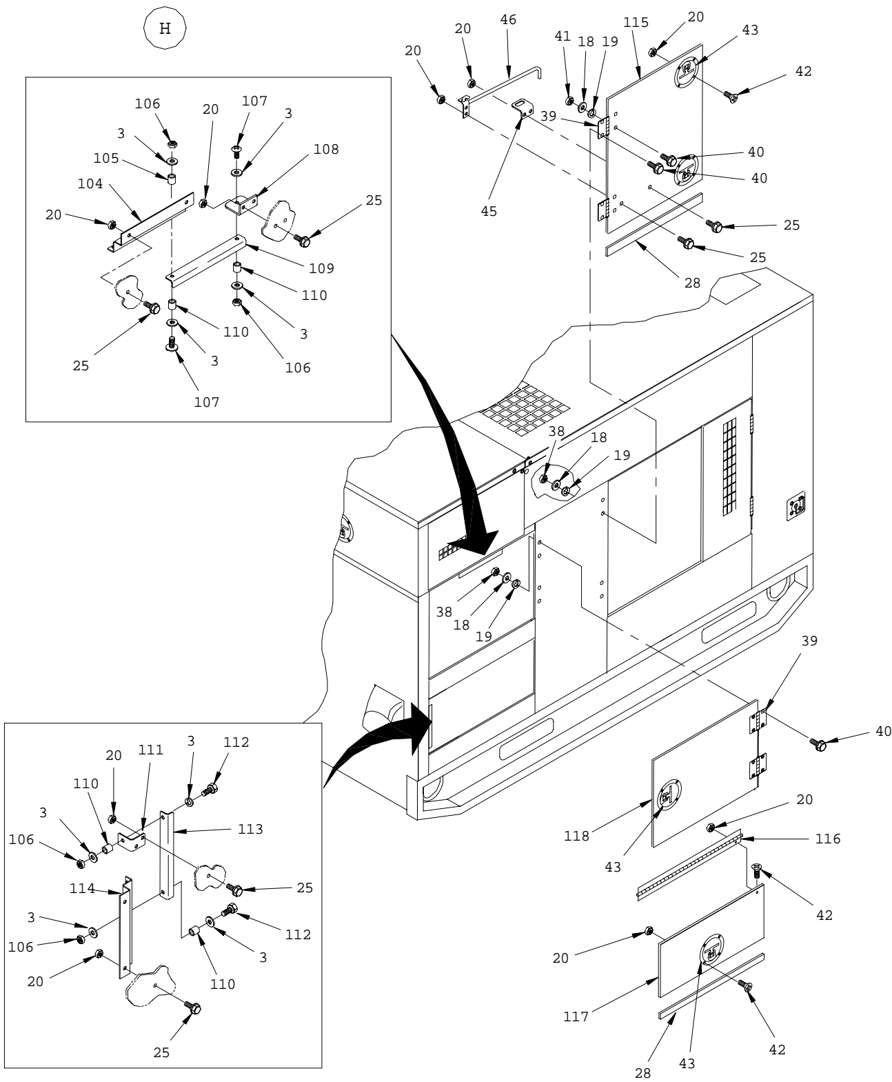
Figure 4. Housing (Sheet 9 of 10)
