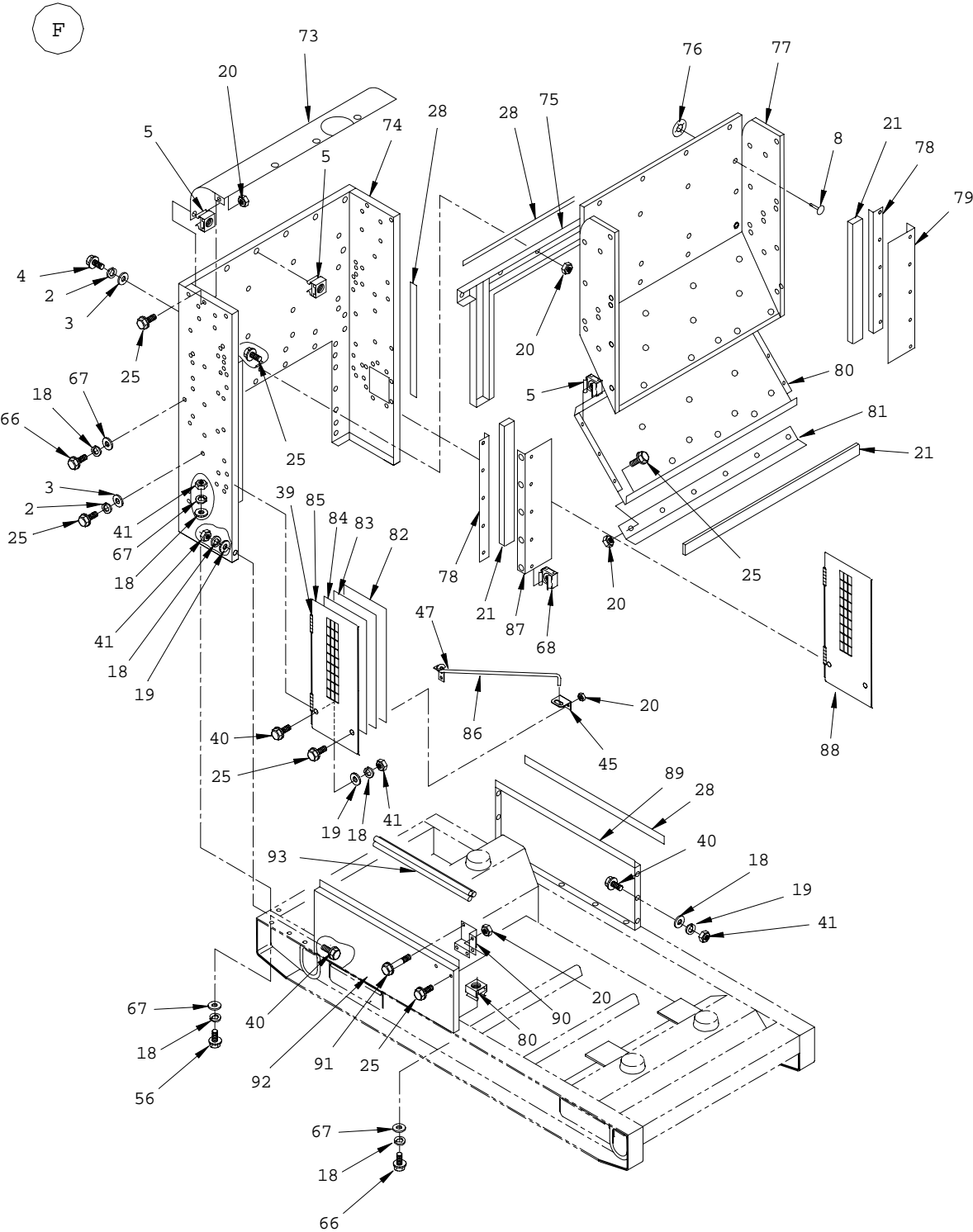
Figure 4. Housing (Sheet 7 of 10)
