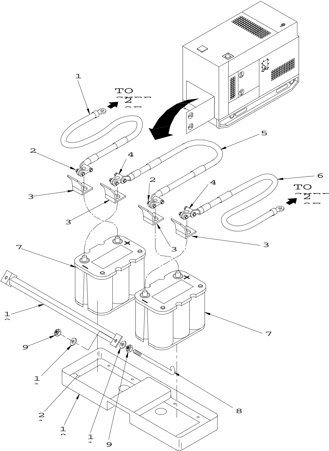
Figure 2. DC Electrical System (Sheet 1 of 2)
